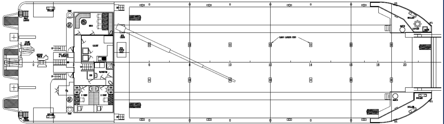
MAIN DECK
